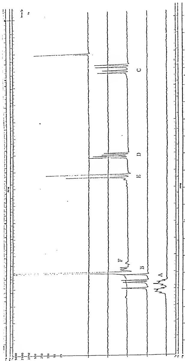
Figure 28 - ^{19}\text{F} NMR of
